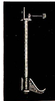
Style L holds radiator 1 7/8 inches from wall.
