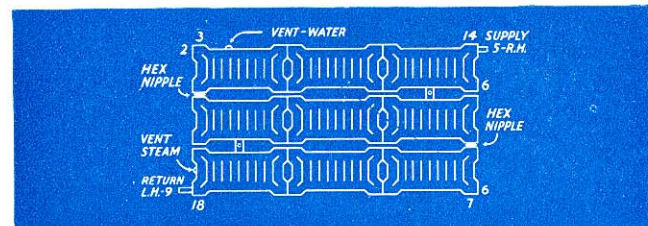
Fig. 17. Assembled nine sections in three tiers. Using adjustable spacing saddle.
