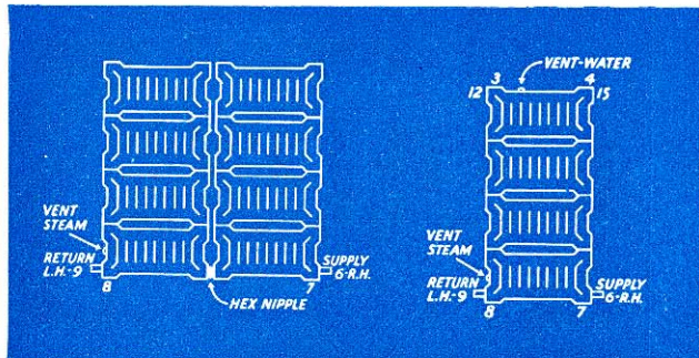
Fig. 13. Assembled in two or more stacks. One and two pipe steam only. Bottom feed.
