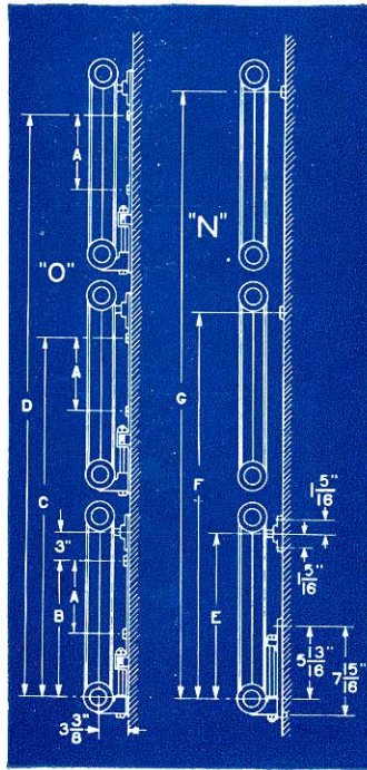
Triton Adjustable Brackets for Wall Radiation
