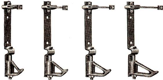
Adjustable, concealed; made to support 3, 4, 5, and 6 tube Capitol wall-hung radiators.
