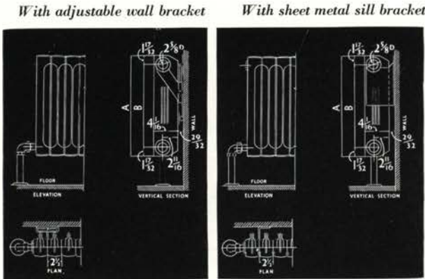
17-INCH HEIGHT, MEASUREMENT A, 17 1/4"; B, 13 1/8" 23-INCH HEIGHT, MEASUREMENT A, 22 1/8"; B, 19 1/8"
