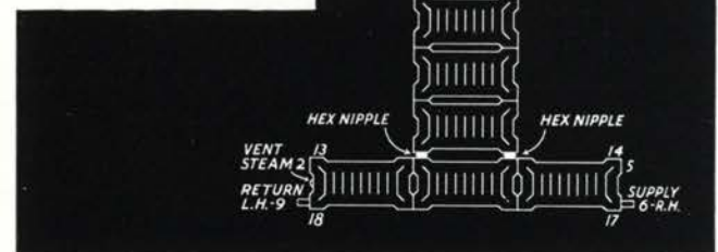
Fig. 15. Assembled in single tier and single stack. Water or one and two pipe steam.
