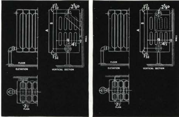
17-INCH HEIGHT MEASUREMENT, A, 17"; B, 13 11/16" 23-INCH HEIGHT MEASUREMENT, A, 22 3/4"; B, 19 11/16"
