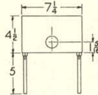
No. 7 Radiator
