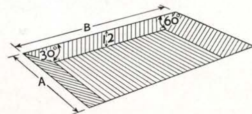
Oil-Burning Type
