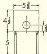
No. 5 Radiator
