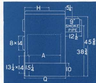
Oil-Burning Type
