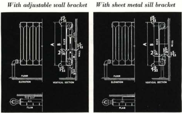
17-INCH HEIGHT, MEASUREMENT A, 17"; B, 14" 20-INCH HEIGHT, MEASUREMENT A, 19 3/4"; B, 16 1/2" 23-INCH HEIGHT, MEASUREMENT A, 22 3/4"; B, 19 3/4"
