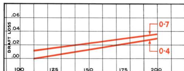
OUTPUT % OF RATED DIRECT CAST IRON RADIATOR LOAD. CURVE BASED ON 12.5% CO 2 .
