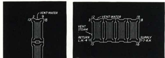
Fig. 2. Assembled in single tier. For water or one and two pipe steam.
