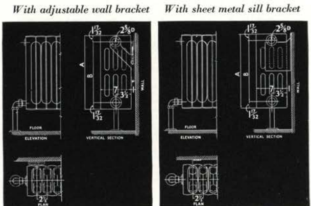
17-INCH HEIGHT, MEASUREMENT A, 17"; B, 13 1/4" 20-INCH HEIGHT, MEASUREMENT A, 20"; B, 16 1/4" 23-INCH HEIGHT, MEASUREMENT A, 22 3/4"; B, 19 1/4"
