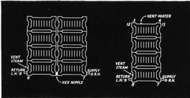
Fig. 13. Assembled in two or more stacks. Fig. 9. Assembled in single stack. One and two pipe steam only. Bottom feed. Water or one and two pipe steam.
